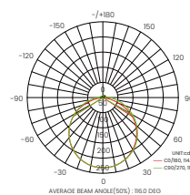
Light Distribution Curve
