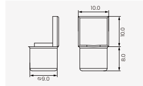
Bottom Cable Entry
