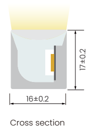
Cross section
