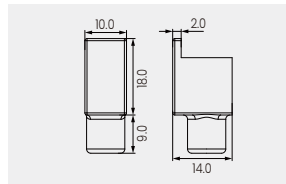
Bottom Cable Entry
