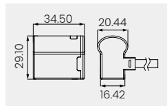
Side Cable Entry
