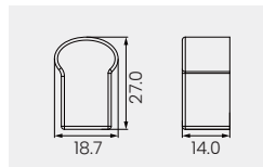
Closed End cap
