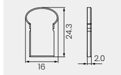
Closed End cap
