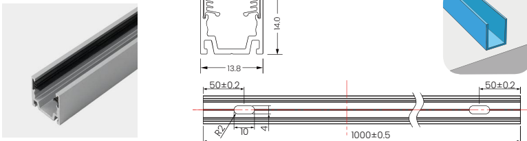
Curved profile : 1213
