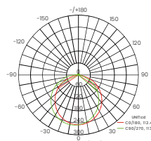
Light Distribution Curve
