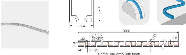
Curved profile
