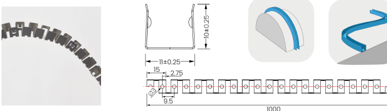
Curved profile
