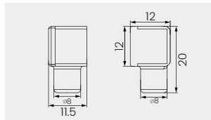
Side Cable Entry
