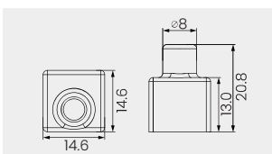
Front Cable Entry
