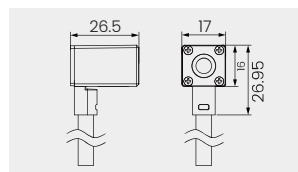
Bottom Cable Entry
