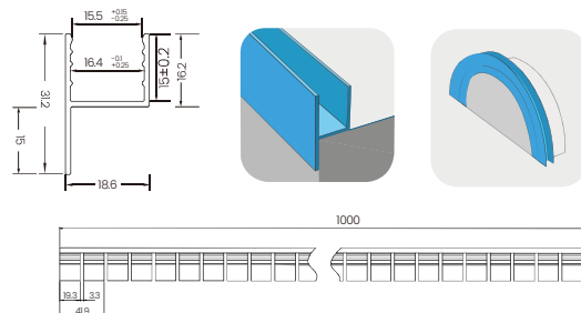
Wing-designed Mounting Channel (Vertical)
