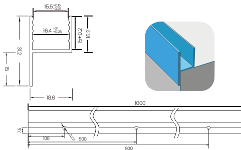
Wing-designed Mounting Channel (Straight)
